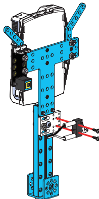
Micro Switch Self-drilling Screw (2)
